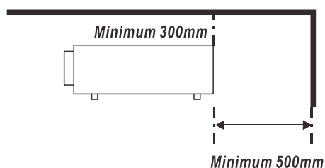
REAR
